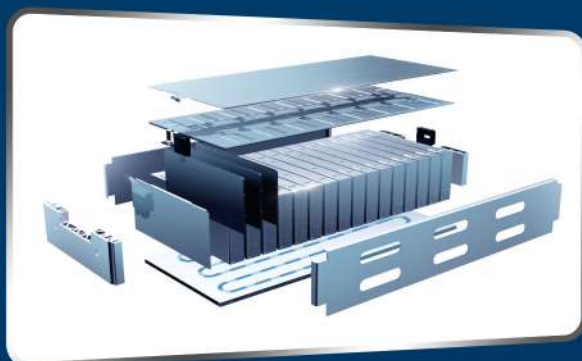
Magazine Battery
